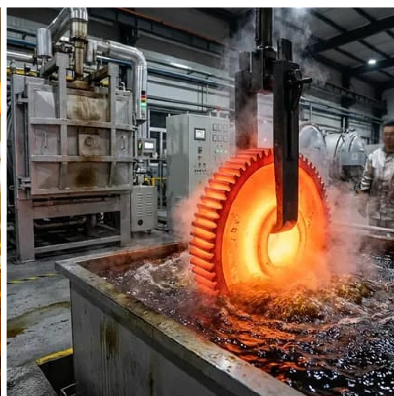
Quenching oil
